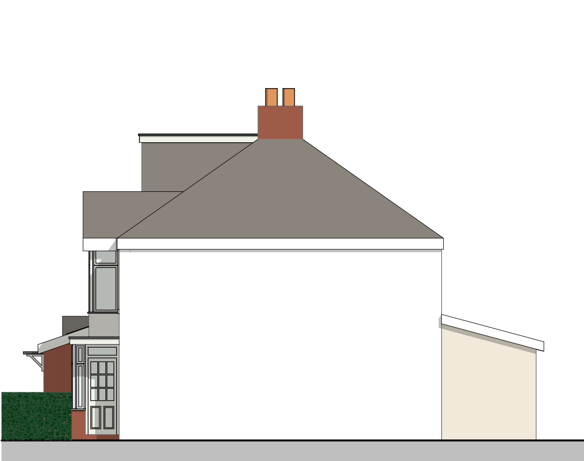
E-02 Existing West Elevation 1:100
