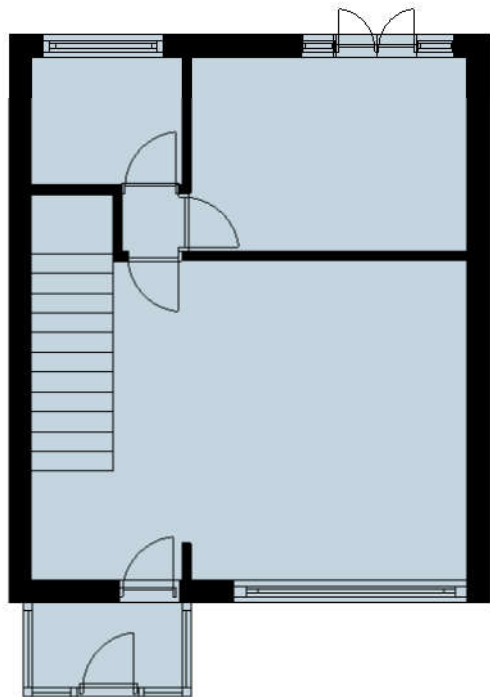
A 13 Proposed Ground Floor 1:100
