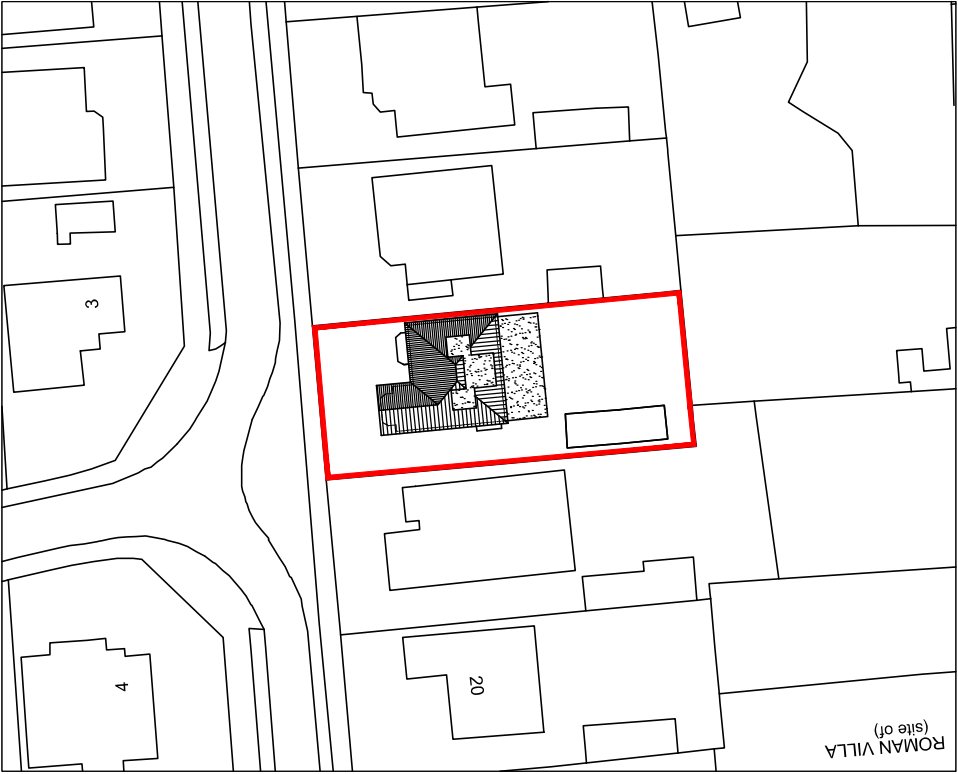
Block Plan: 1:500
