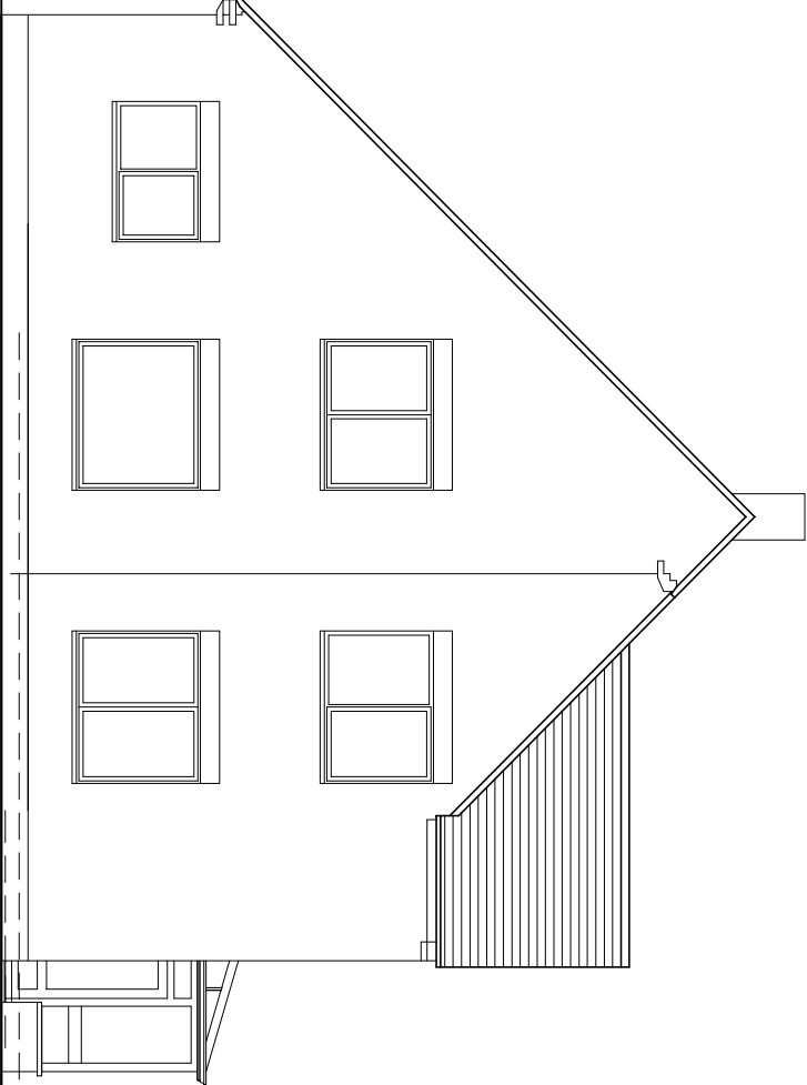
West Elevation
