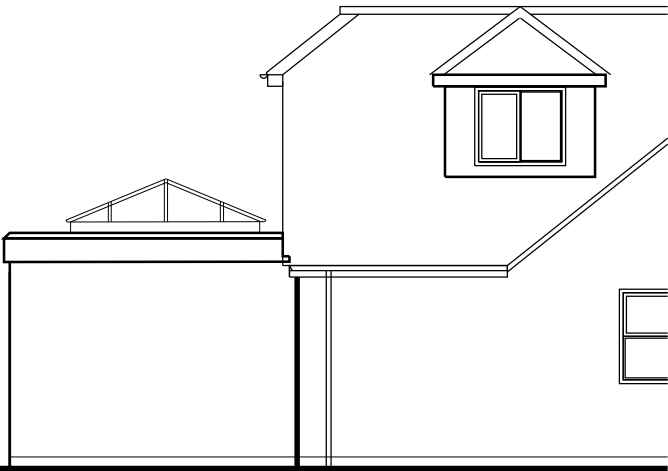
West Elevation
