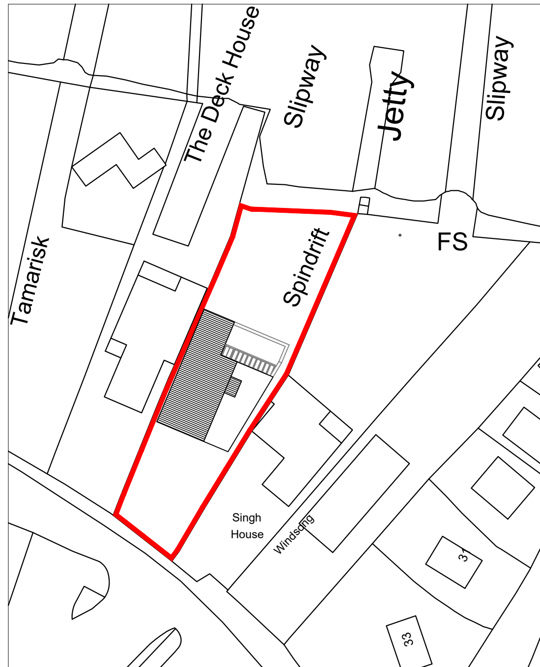
Block Plan: 1:500
