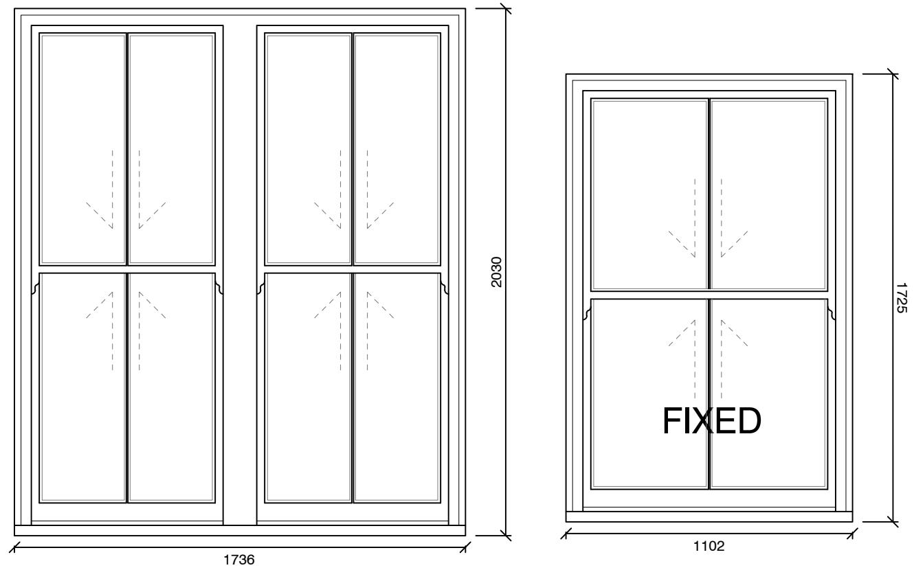
WINDOW W1.02 Double Sash 1:20
