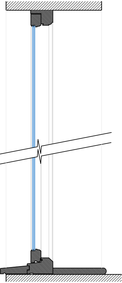
WINDOW Section W.02 Timber Frame 1:10
