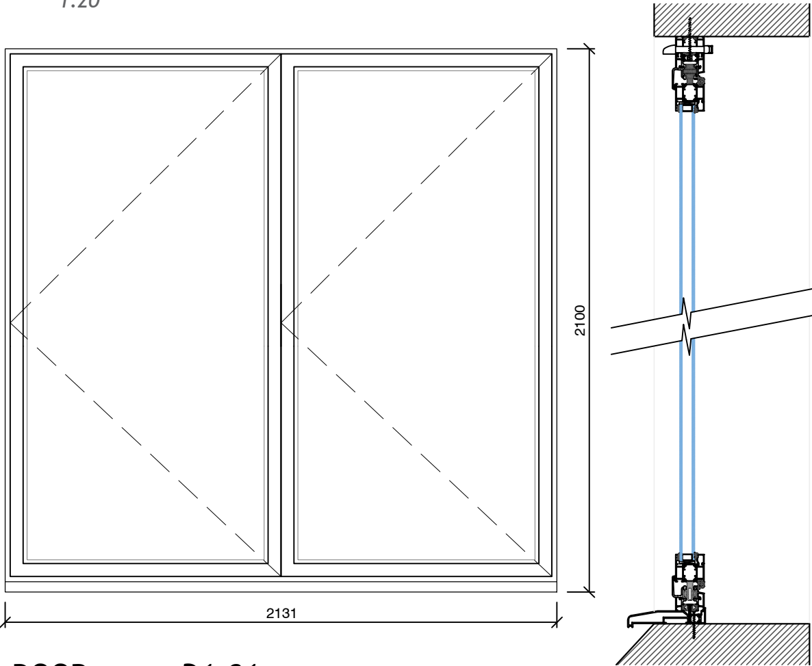
DOOR D1.01 Aluminium Frame Bi-fold 1:20
