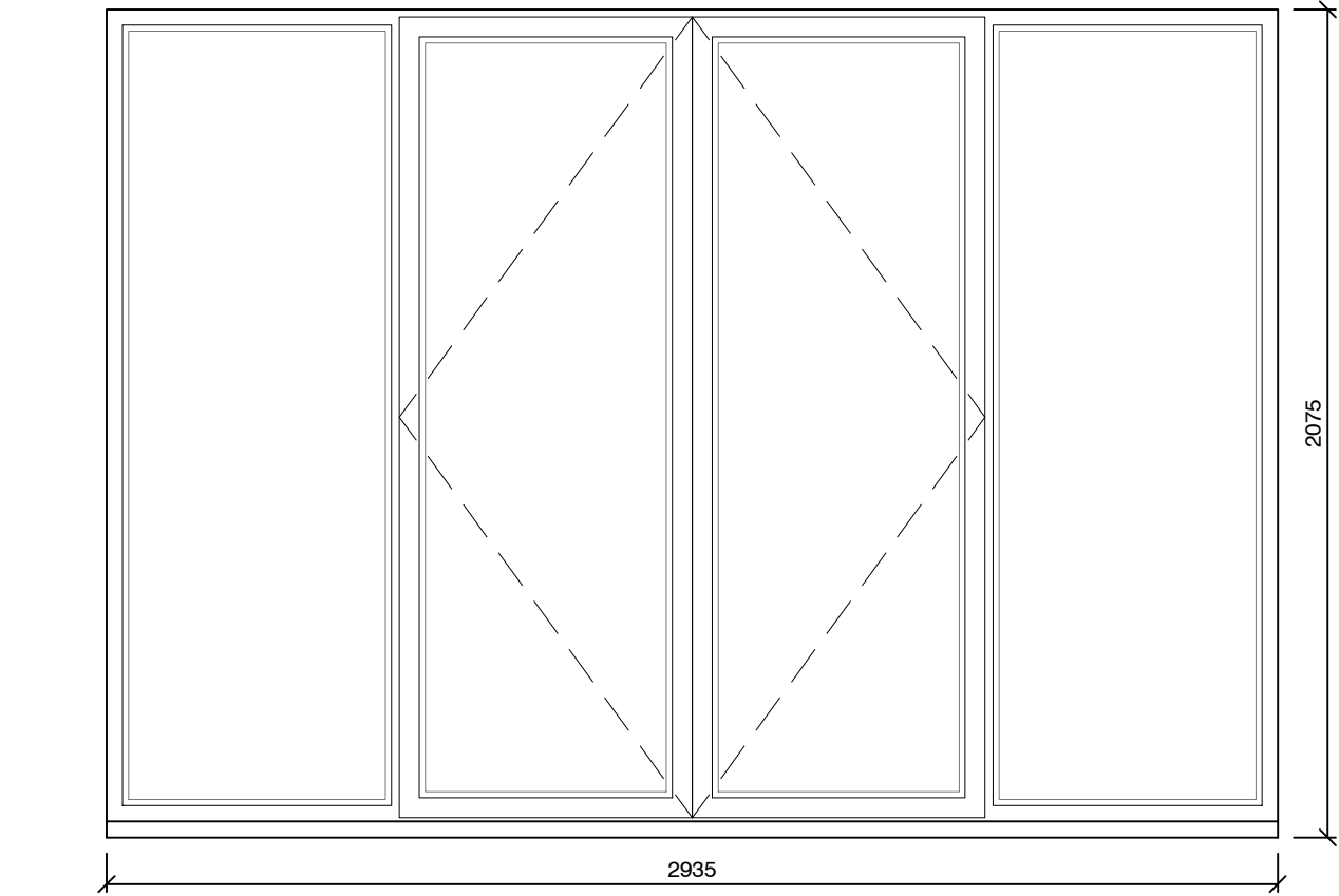
WINDOW W.02 Central french double doors with fixed side lights - Timber Frame 1:20
