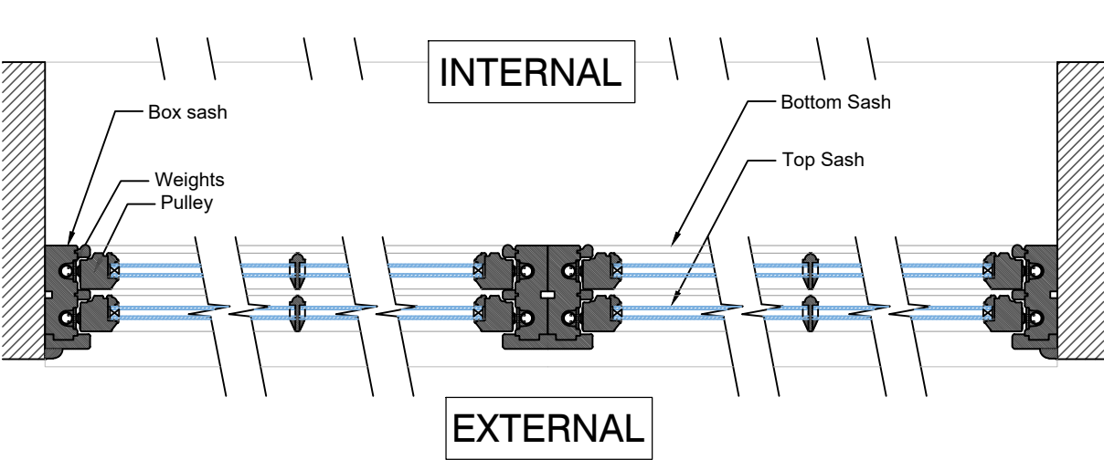
Sash Box Window Horizontal Section (For Sash Window W1.02, W2.03 & W3.01) 1:10
