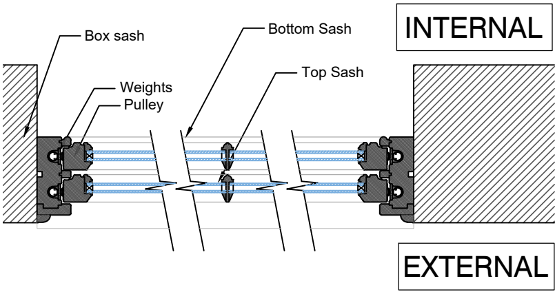
Sash Box Window Horizontal Section (For Sash Window W2.01) 1:10
