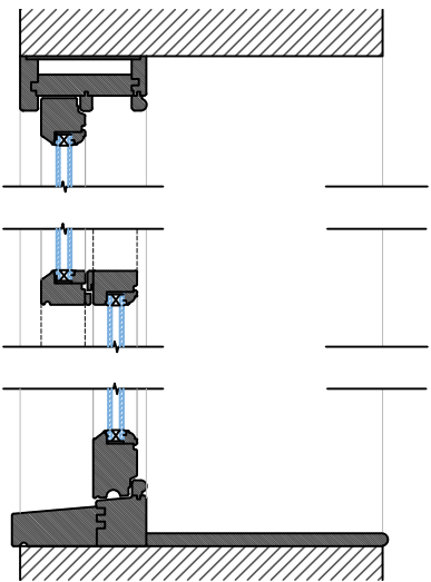
Sash Box Window Section (For Sash Window W1.02, W2.01, W2.03, W3.01) 1:10
