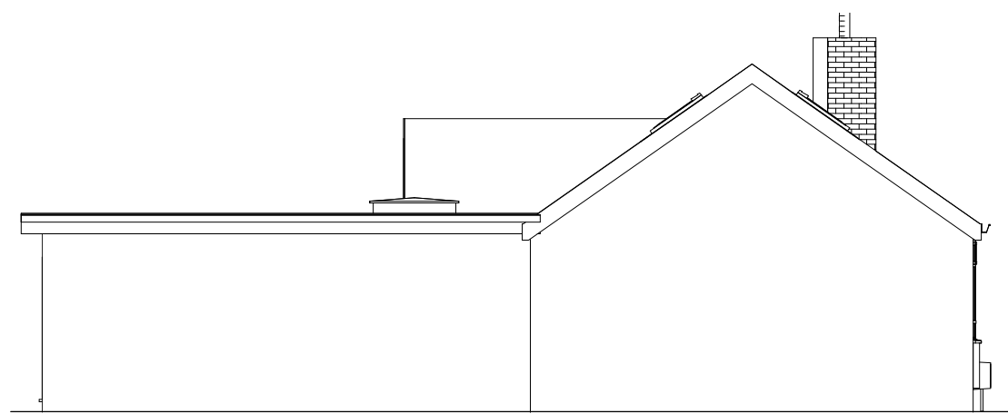
2 North Elevation 1 : 100
