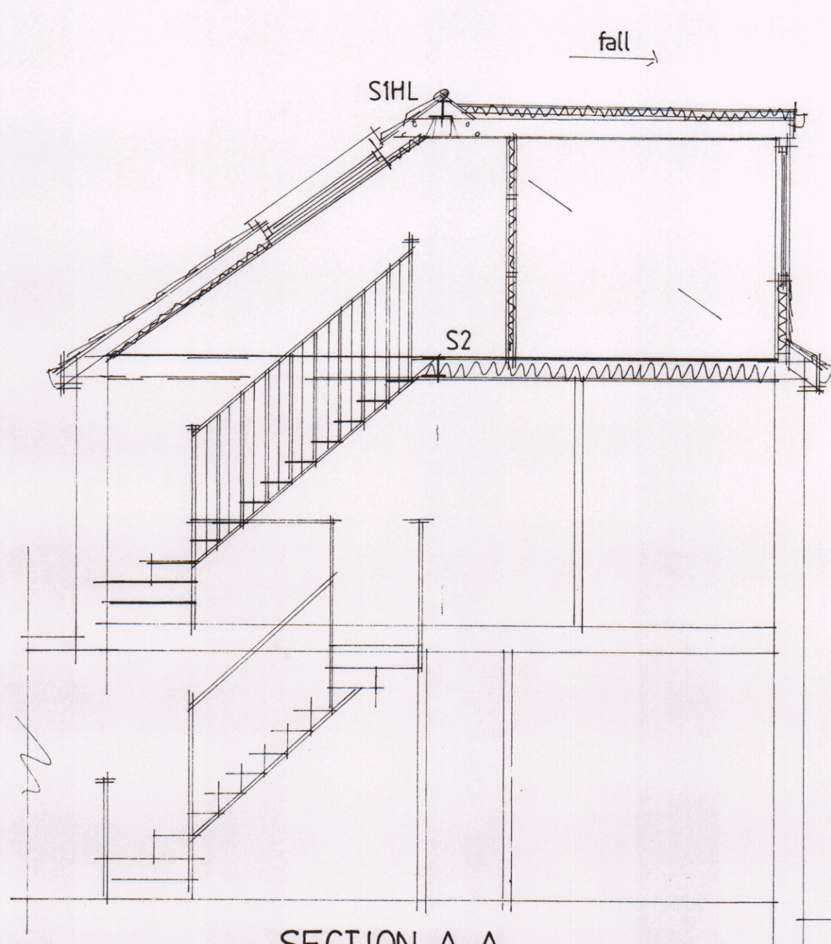
SECTION A.A.
