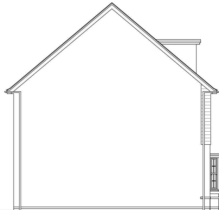
SIDE ELEVATION 1
