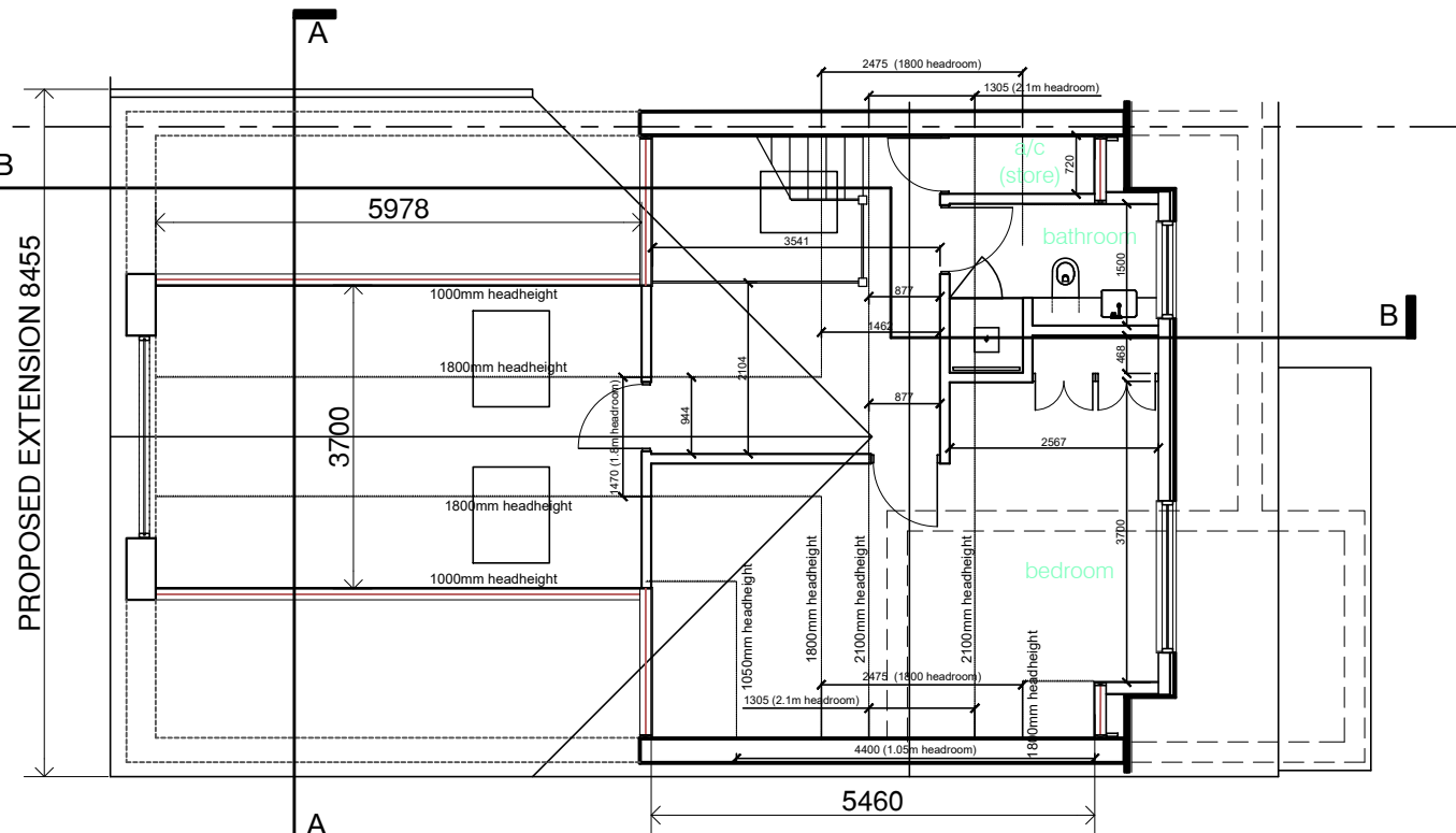
PROPOSED FIRST FLOOR scale 1:100 @ A3 1:50 @ A1
