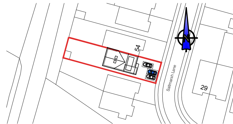
PROPOSED SITE PLAN scale 1:1000 @ A3 1:500 @ A1
