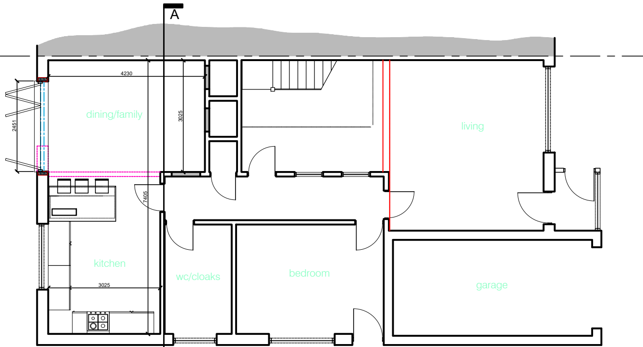
PROPOSED GROUND FLOOR scale 1:100 @ A3 1:50 @ A1
