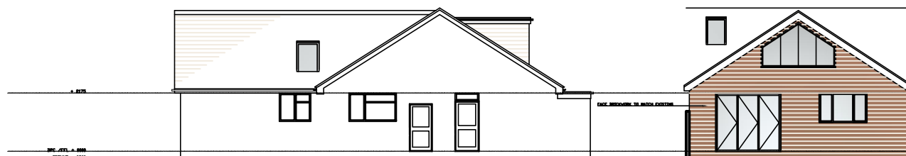
PROPOSED REAR ELEVATION
