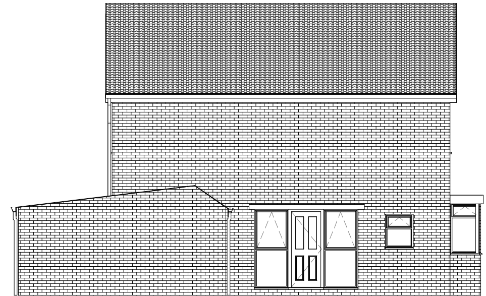
2 North Elevation 1 : 100
