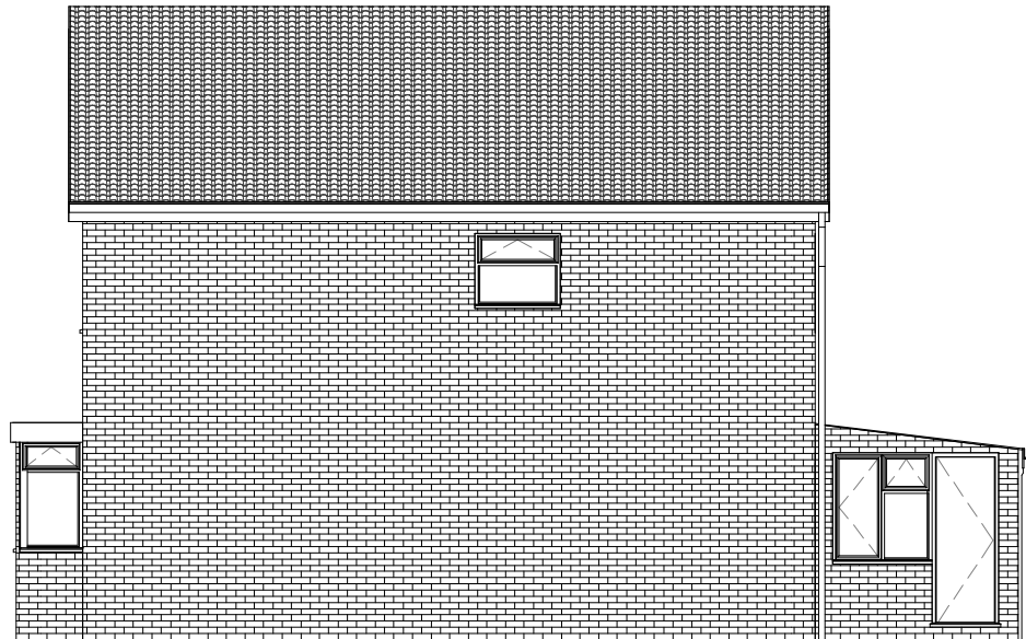
3 South Elevation 1 : 100
