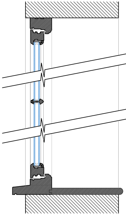
Casement Window Section (For Windows W.01 & W.03) 1:10
