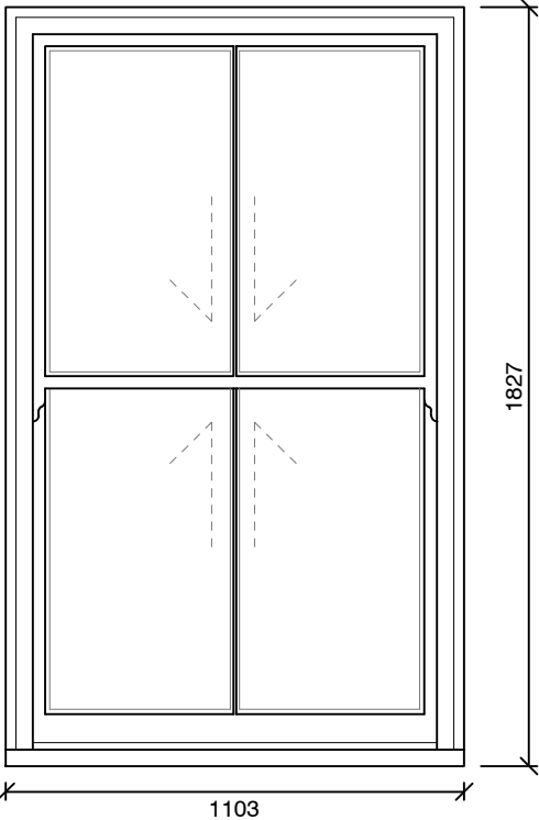
WINDOW W2.02 Sash 1:20
