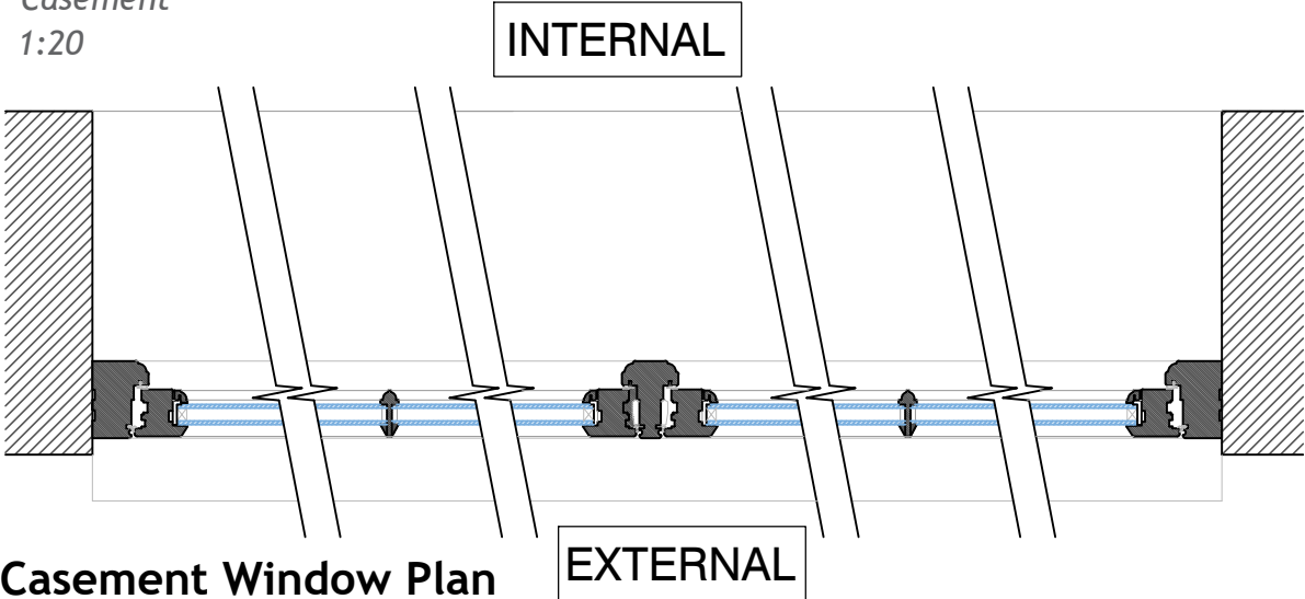
Casement Window Plan (For Window W.01 & W.03) 1:10
