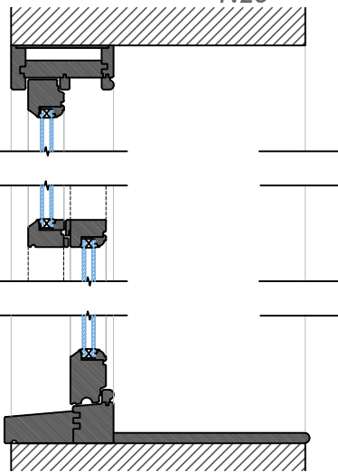
Sash Box Window Section (For Sash Window W1.01 & W2.02) 1:10
