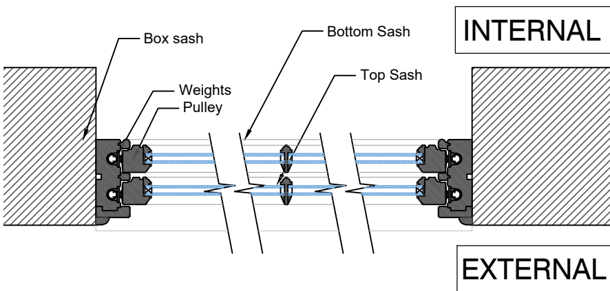
Sash Box Window Plan (For Sash Window W2.02) 1:10
