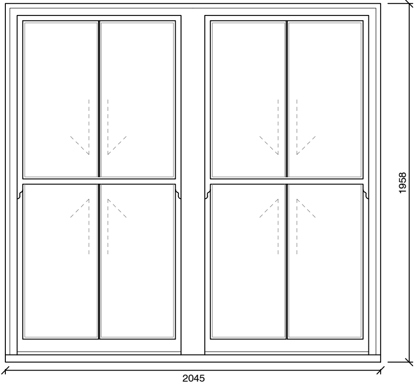
WINDOW W1.01 Sash 1:20
