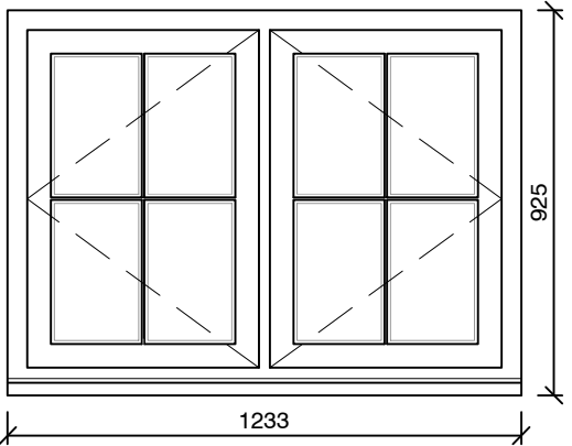
WINDOW W.03 Casement 1:20
