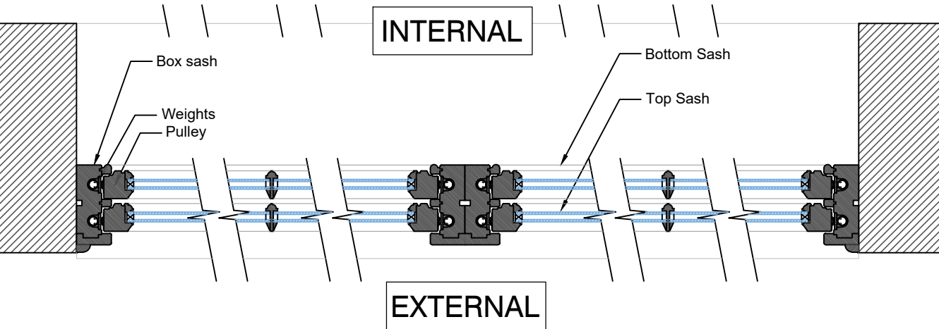
Sash Box Window Plan (For Sash Window W1.01) 1:10
