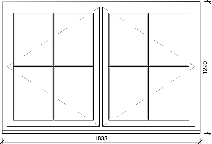
WINDOW W.01 Casement 1:20
