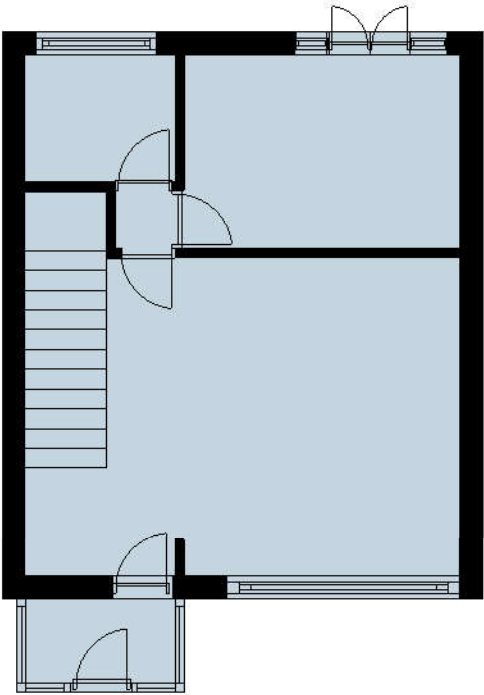
A 7 Ground Floor Plan 1:100
