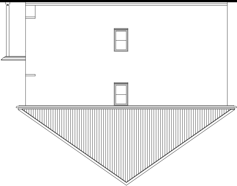
SIDE ELEVATION 1
