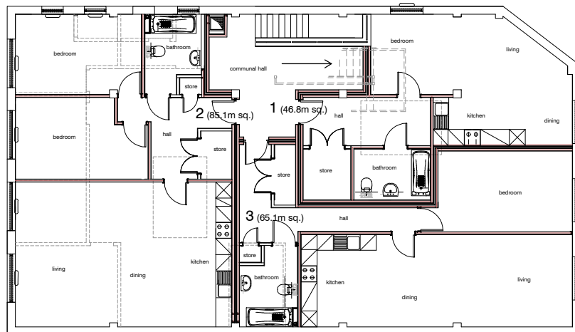
Proposed First Floor Plans
