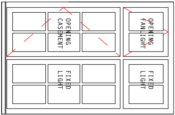
WINDOW 1 WINDOWS WITH TIMBER GLAZING BARS 12 DOUBLE GLAZED UNITS
