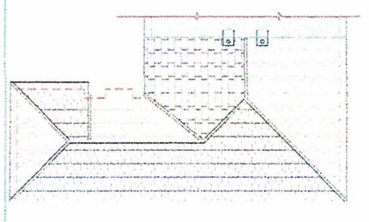
6 EXISTING ROOF PLAN 1:100
