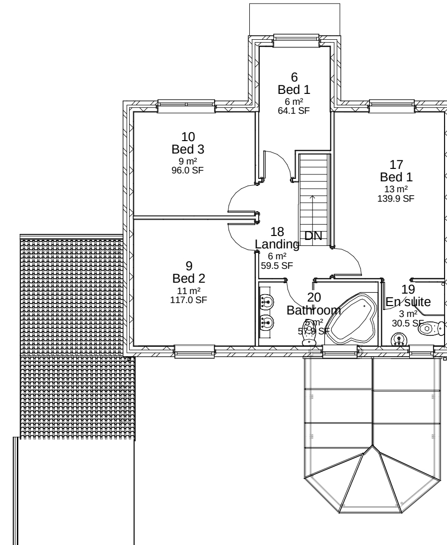
2 First Floor 1 : 100
