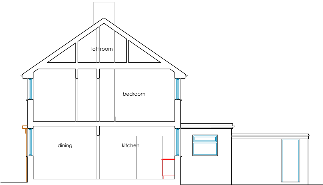
Section AA
