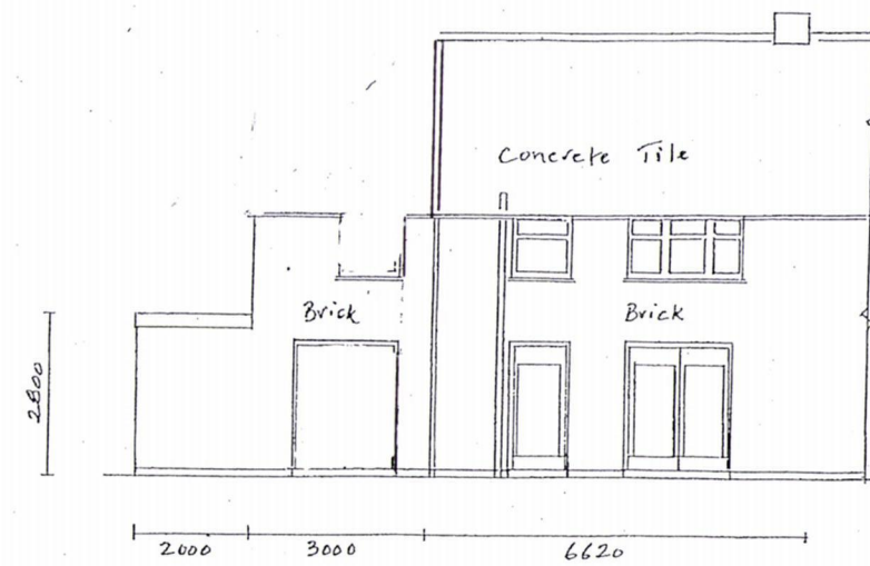
REAR - EXISTING NORTH ELEVATION
