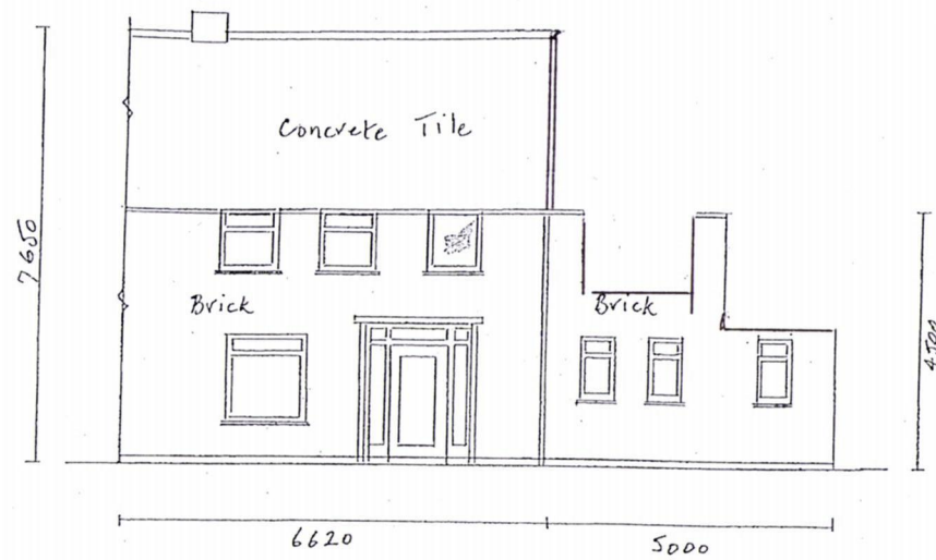
FRONT - EXISTING SOUTH ELEVATION
