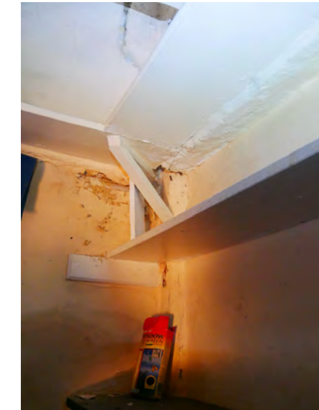
40. SE corner of G17, concealed jowl post, with cross beam evident. The side girt can be found above the top shelf.
