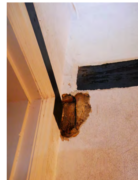
39. SE corner of G15 - evidence of side girt. The cross beam is likely to be reused from the dismantled frame.
