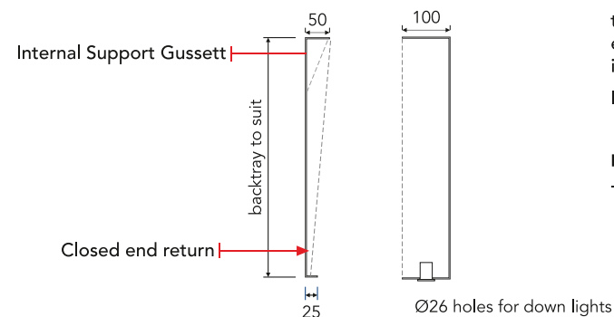
A-A Section Detail Scale 1:10
