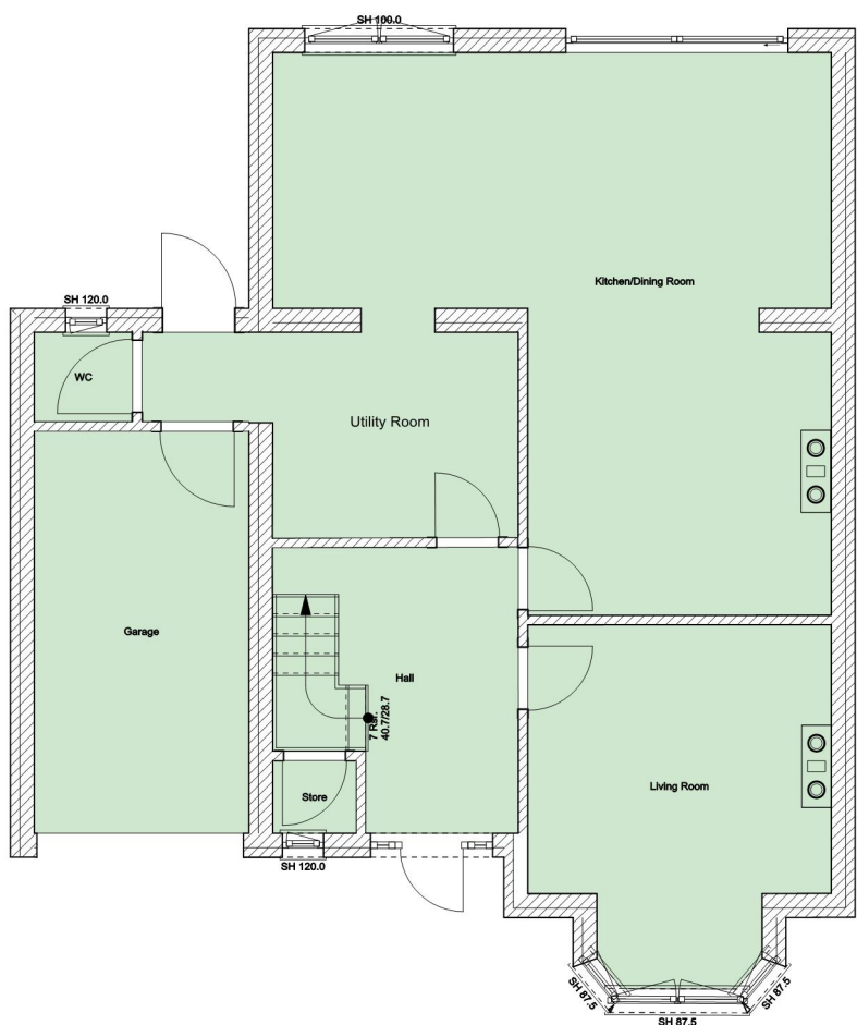
Ground Floor Proposed Floor Plan
