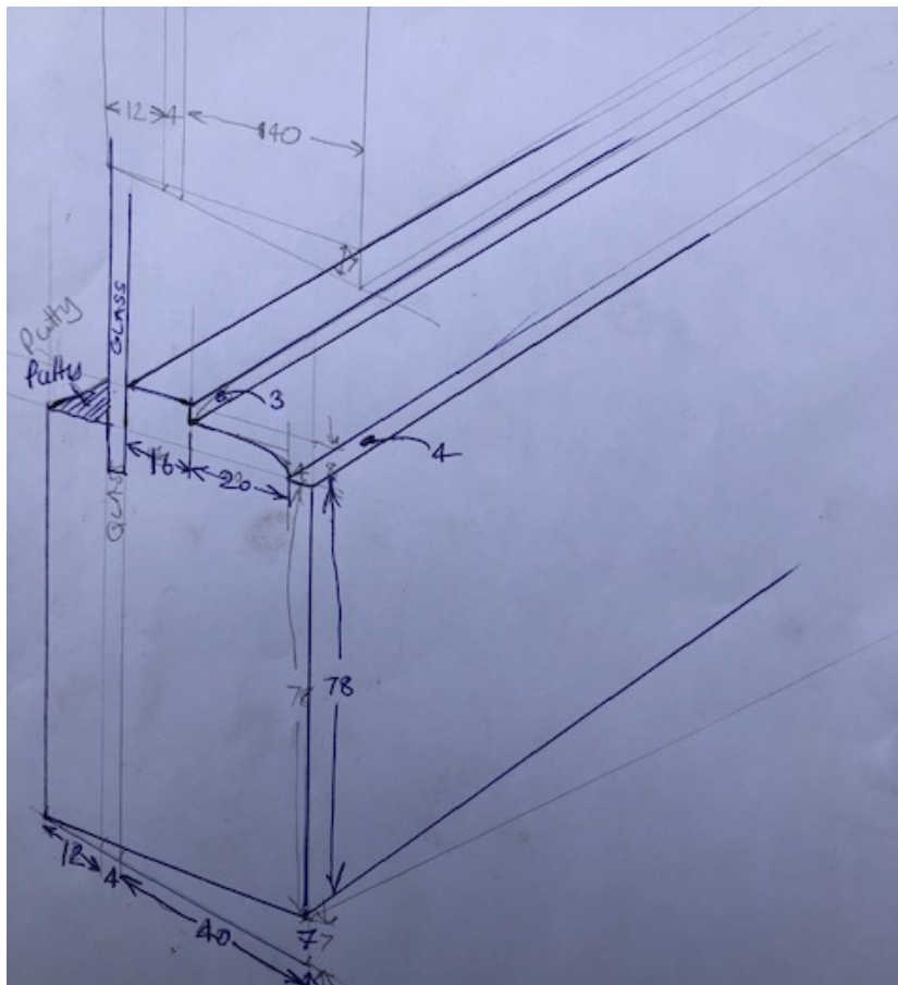
Lower Sash with Puttied Bead, Single Glazing
