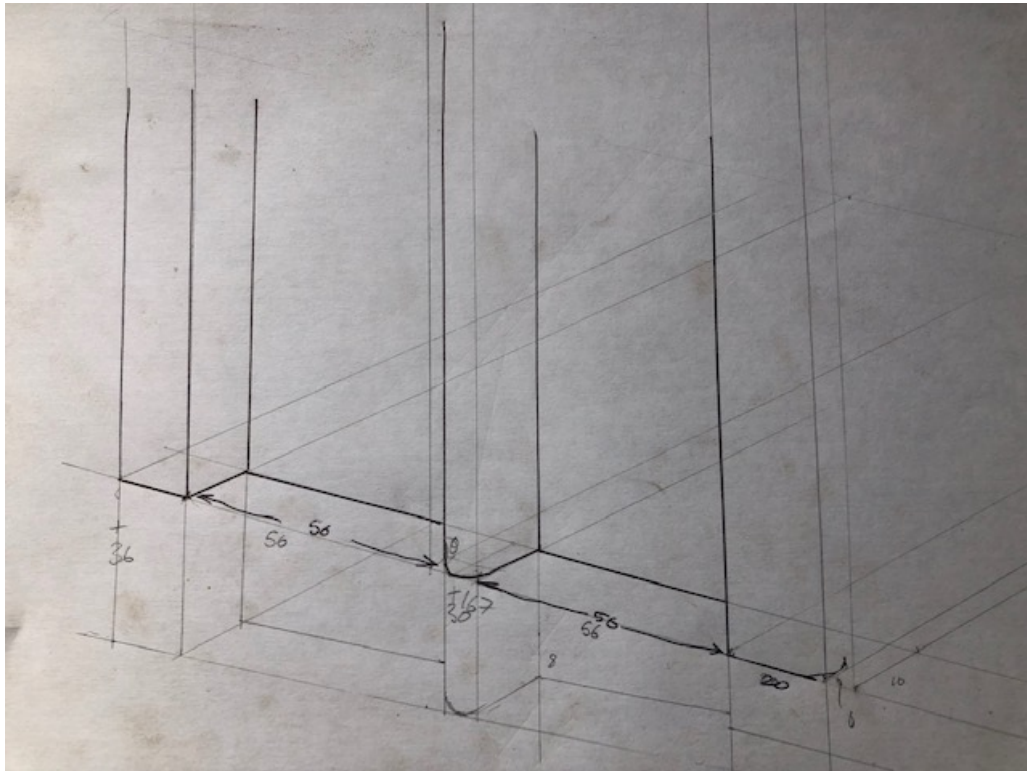
Cross Section Frame Uprights
