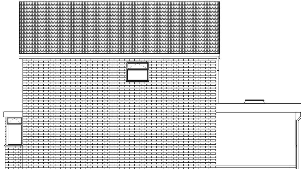
3 South Elevation 1 : 100
