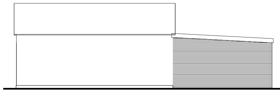
1 East Garage Elevation 1 : 100
