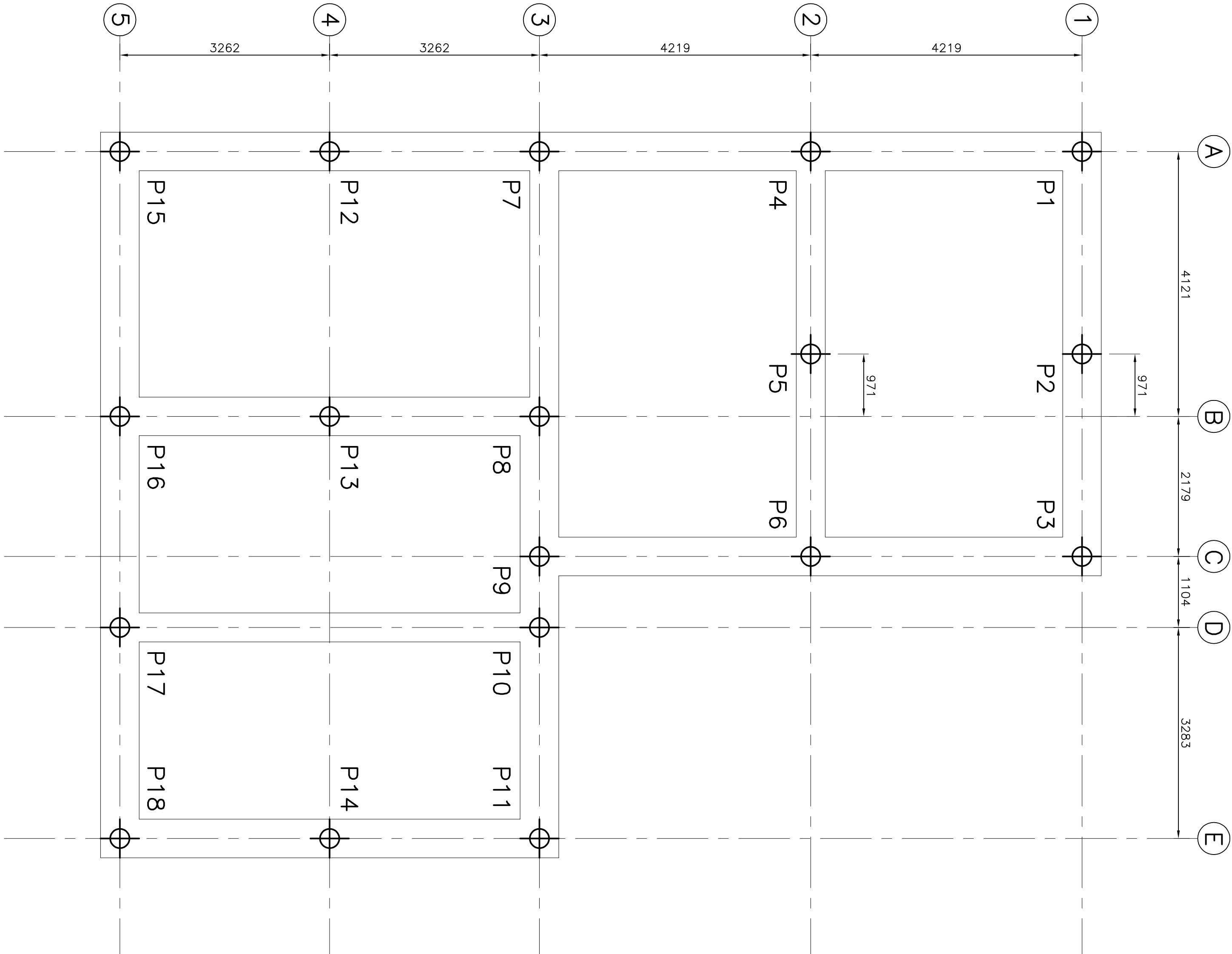
PLOT 1 PILE LAYOUT 1:50
