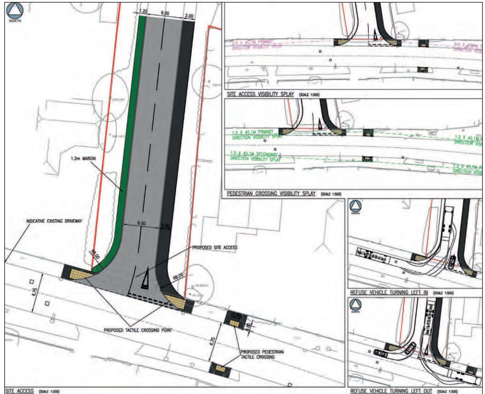
Proposed Access Road Plan (prepared by Paul Basham Associates)
