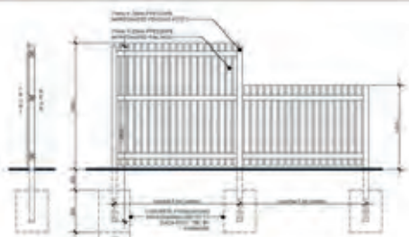
1800mm Timber Close Boarded Fence reduced to 1200mm after 2m from rear wall.
