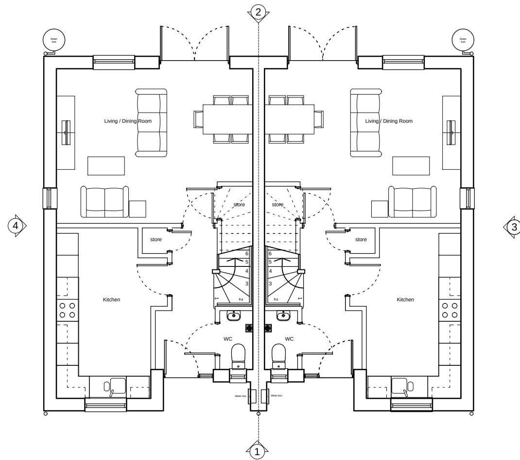
01 Ground Floor Plan 2004 Scale: 1:100
