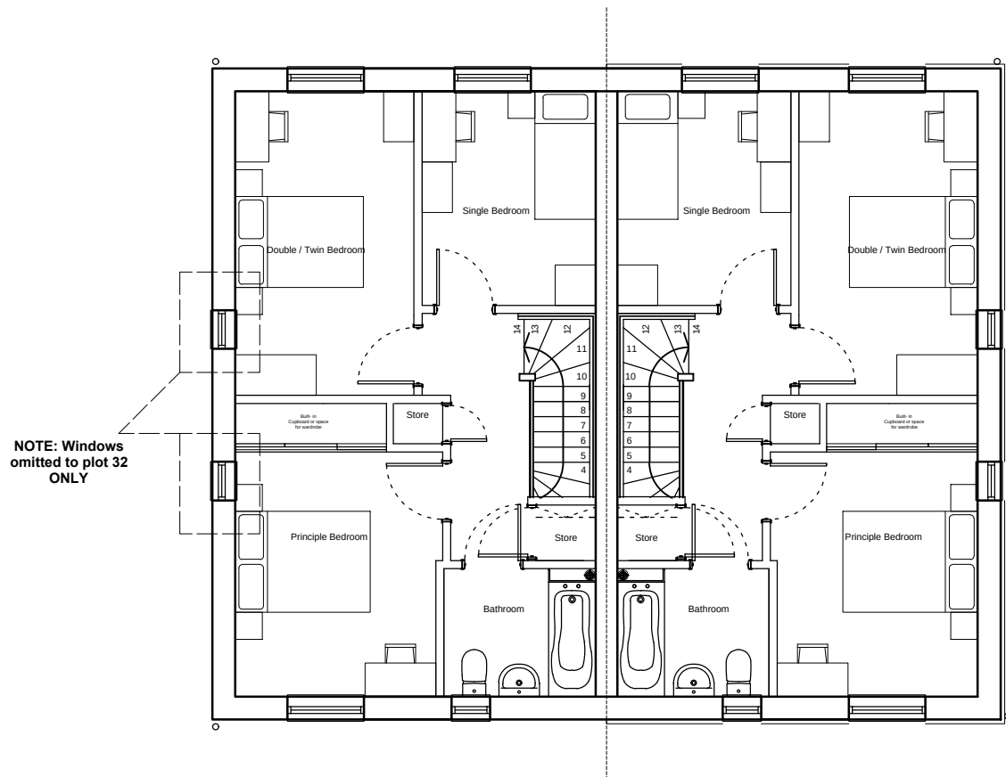
02 First Floor Plan 2004 Scale: 1:100
