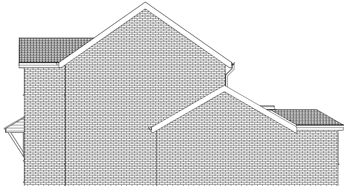
3 South Elevation 1 : 100
