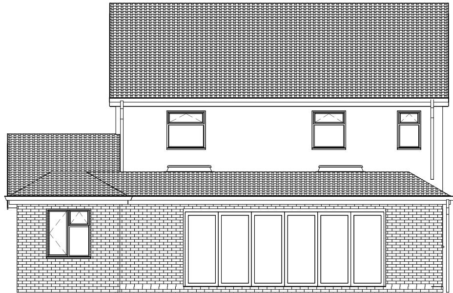
1 East Elevation 1 : 100
