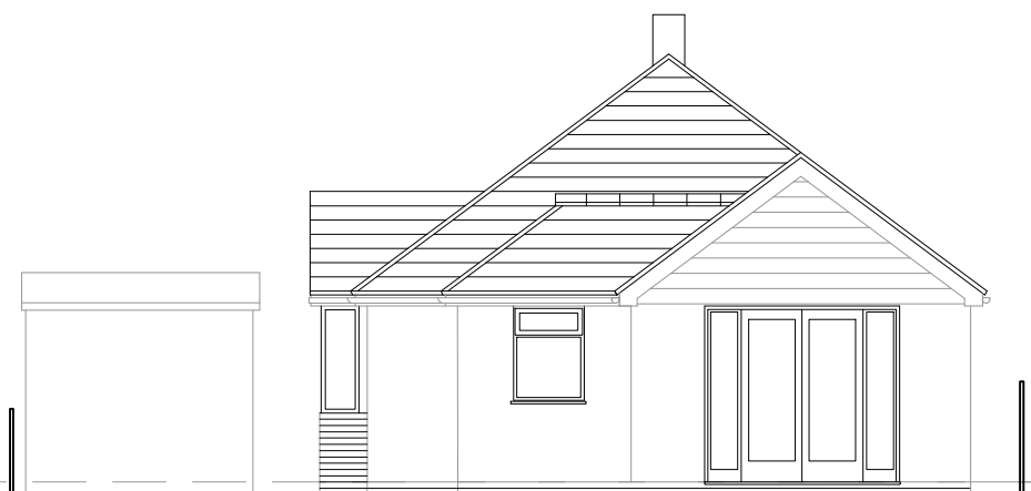
east elevation
