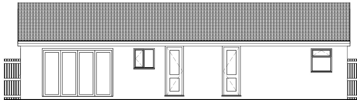
5 West Garage Elevation 1 : 100
