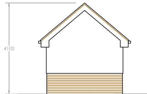
Rear Elevation
