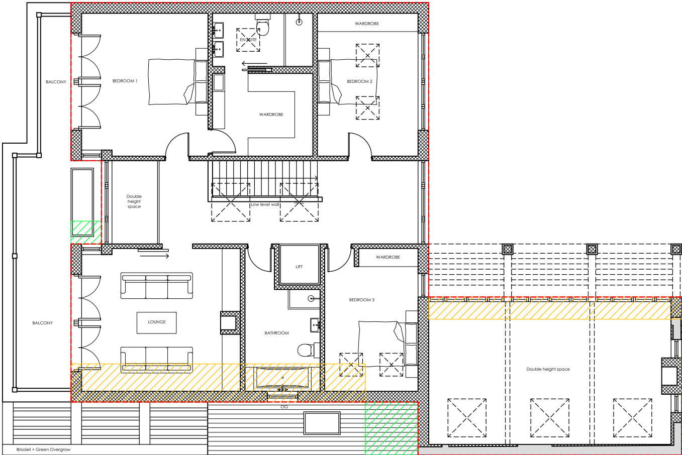
PERMITTED FIRST FLOOR PLAN
