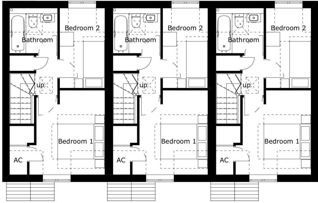
FIRST FLOOR - 1:100
