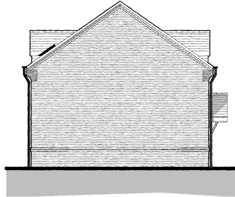
SIDE ELEVATION [1] - 1:100
