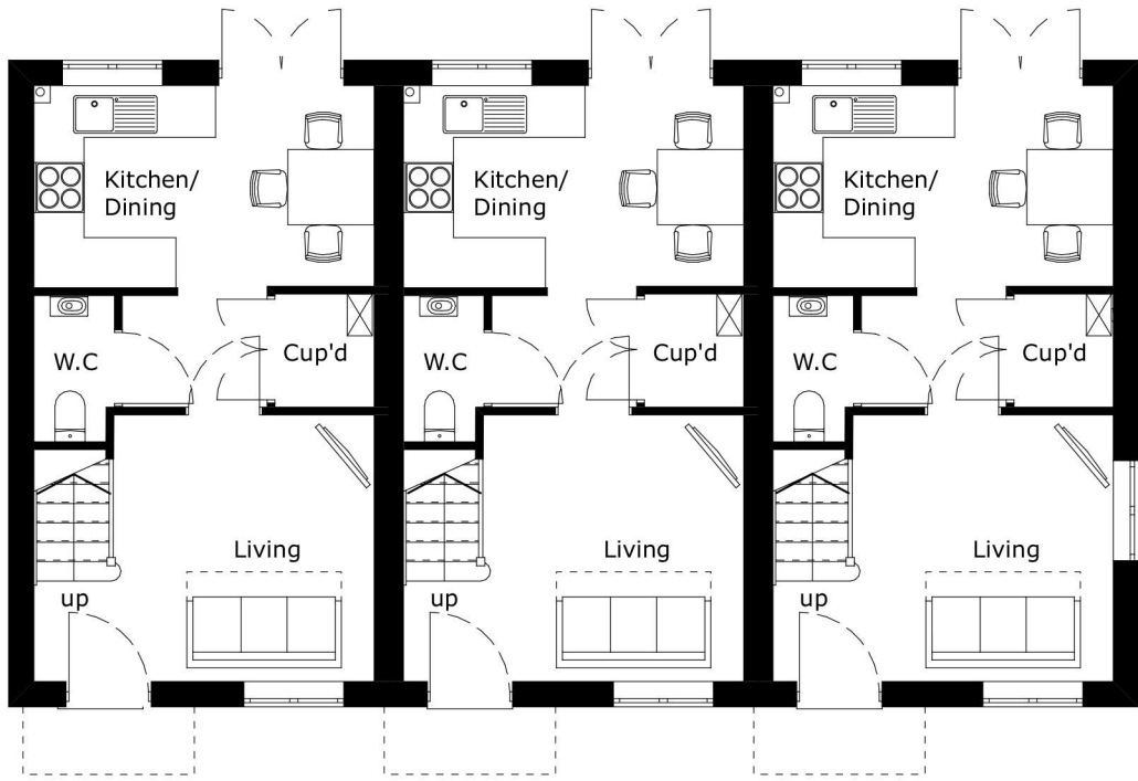
GROUND FLOOR - 1:100
