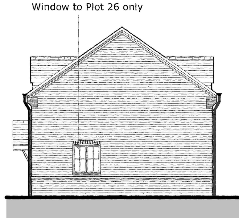
SIDE ELEVATION [2] - 1:100
