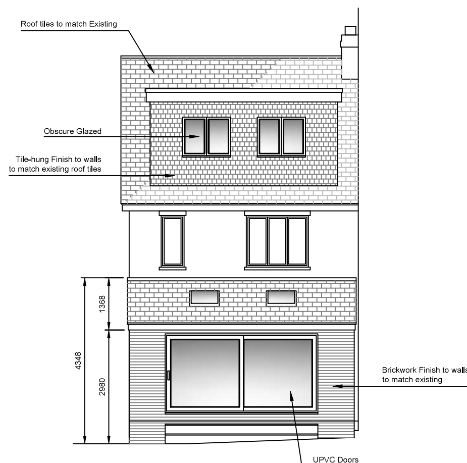
Rear Elevation
