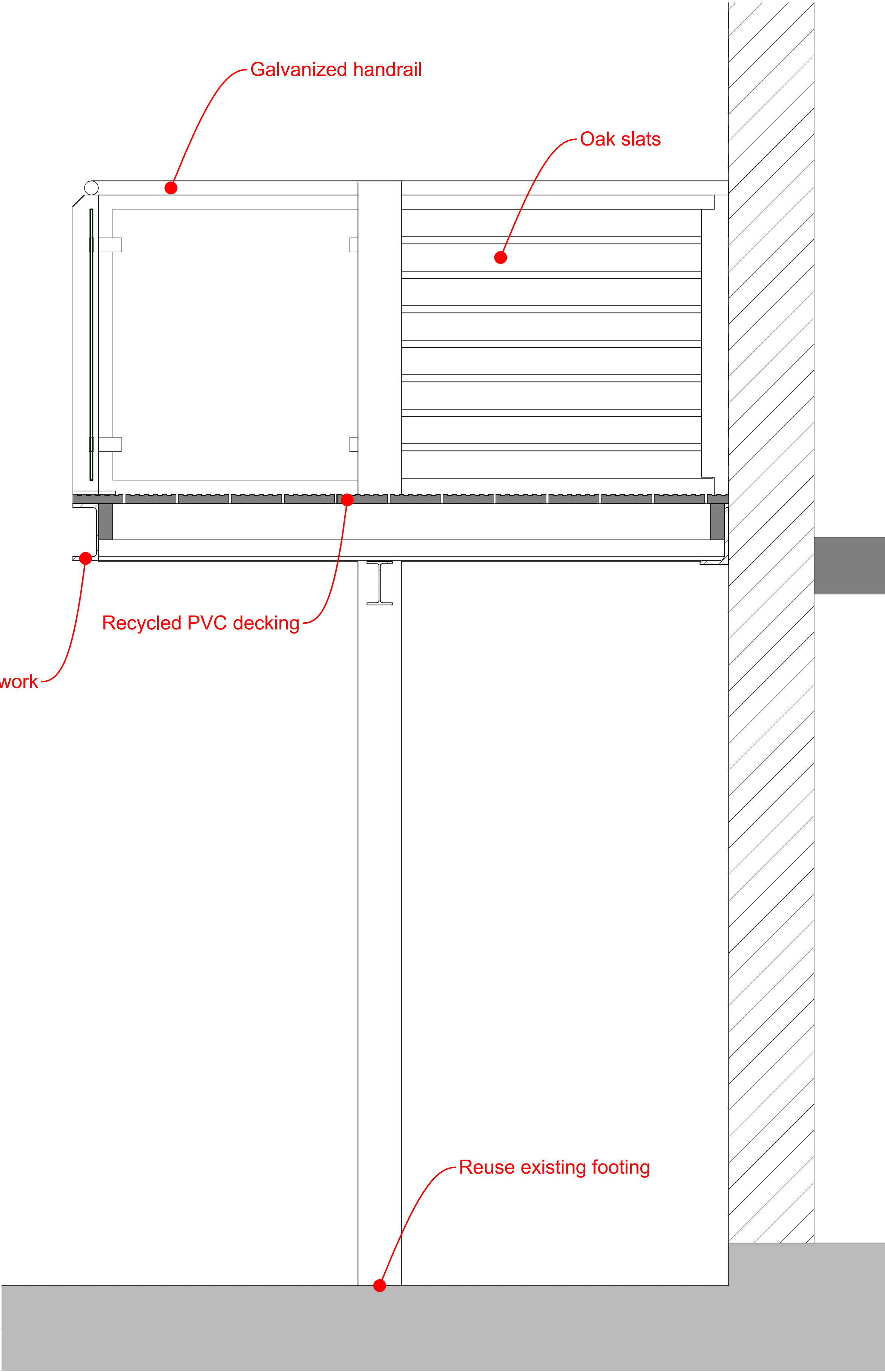
Proposed Section
