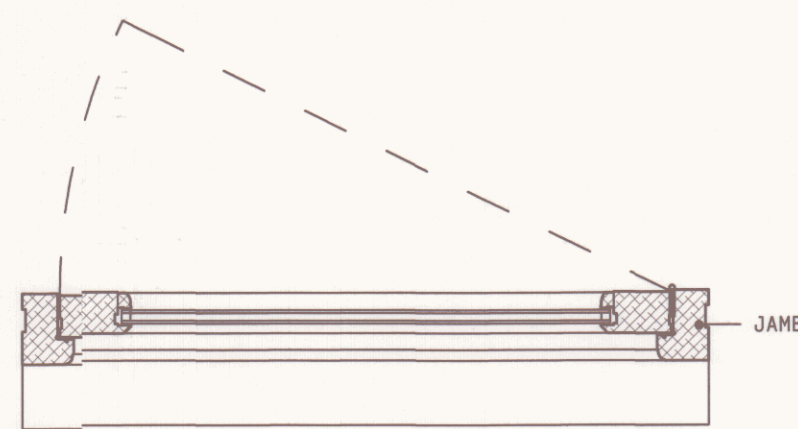
typical door horizontal section
