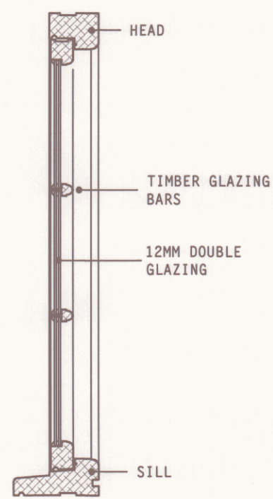
typical window vert section
