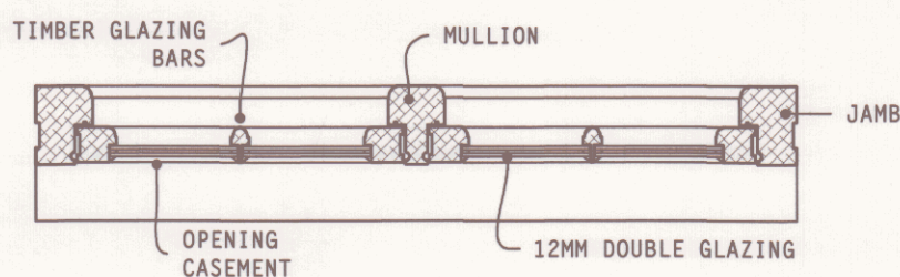
typical window horizontal section
