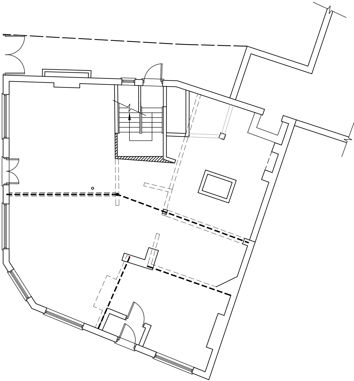
GROUND FLOOR
