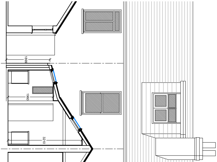
Cross section north - proposed
