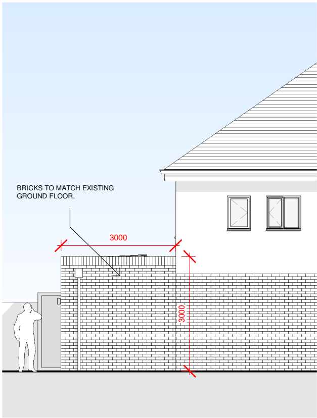
P-005 PROPOSED SIDE ELEVATION 1 : 100
