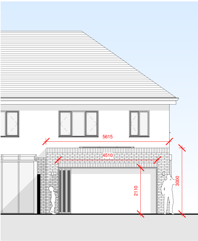
P-005 PROPOSED REAR ELEVATION 1 : 100
