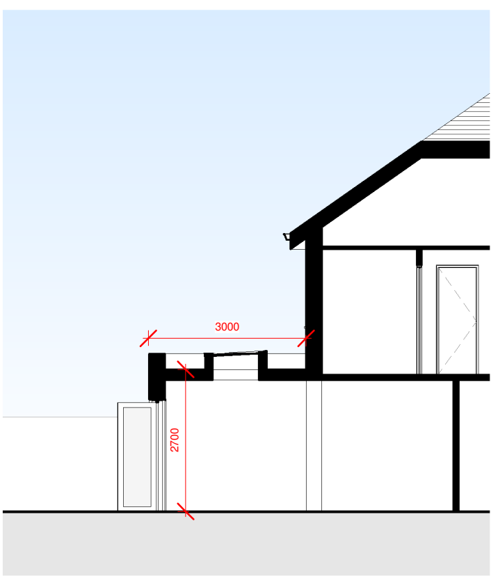
P-005 PROPOSED SECTION 1 : 100
