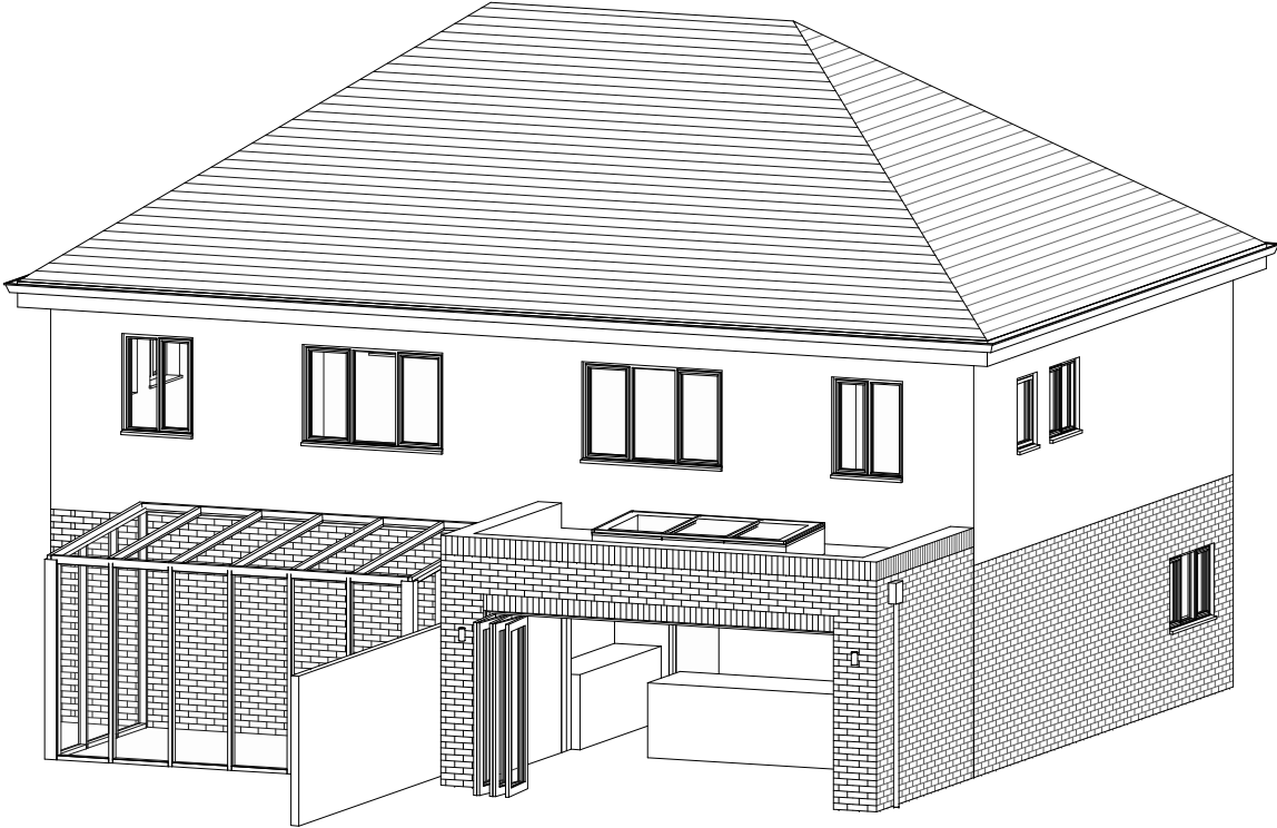
P-005 PROPOSED AXO
