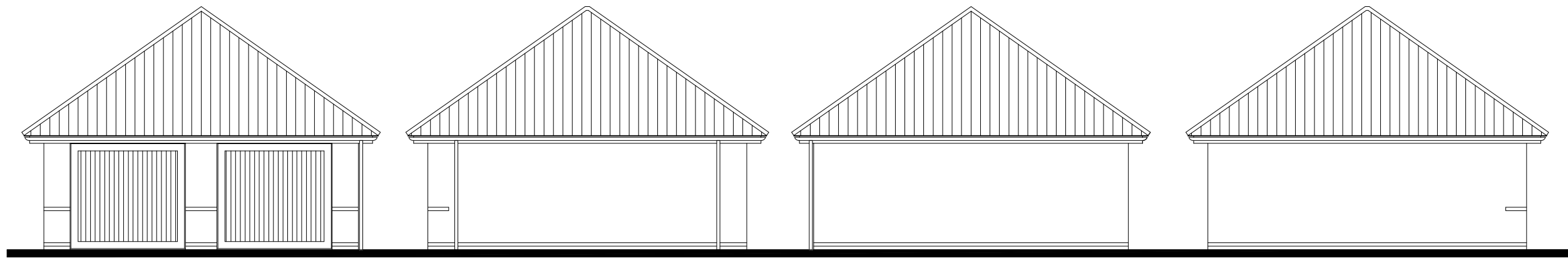
FRONT ELEVATION
