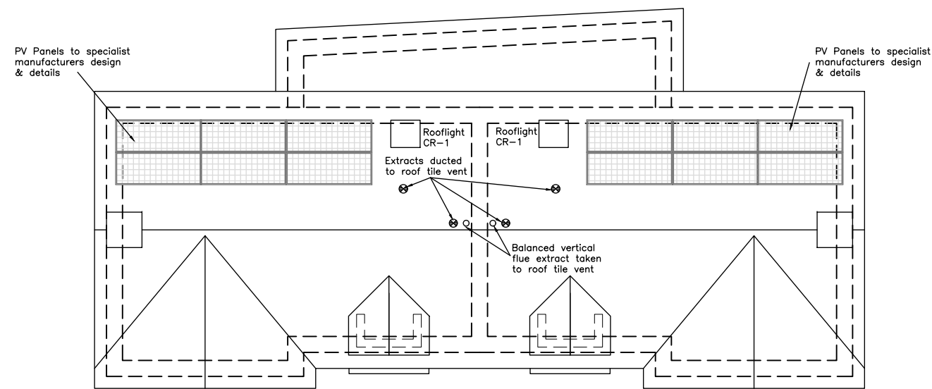
Roof Plan
