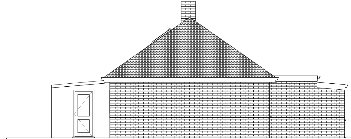
2 North Elevation 1 : 100
