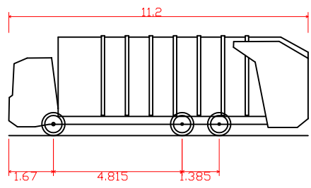
REFUSE VEHICLE
