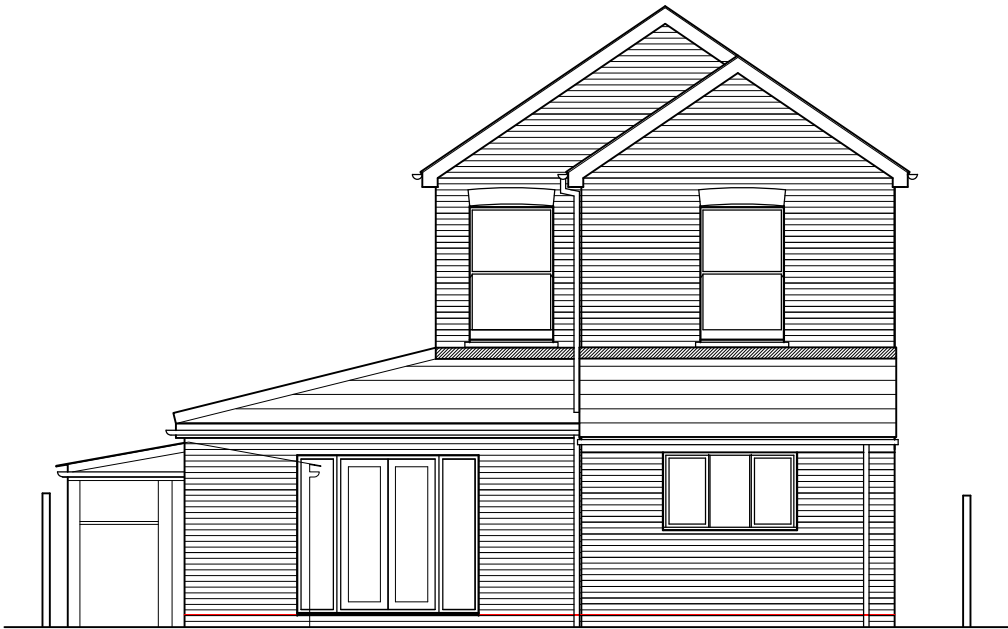
South (rear) elevation
