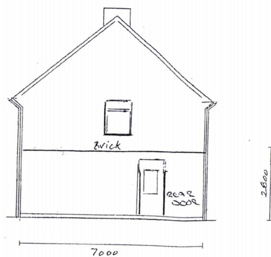
SIDE PROPOSED ELEVATION
