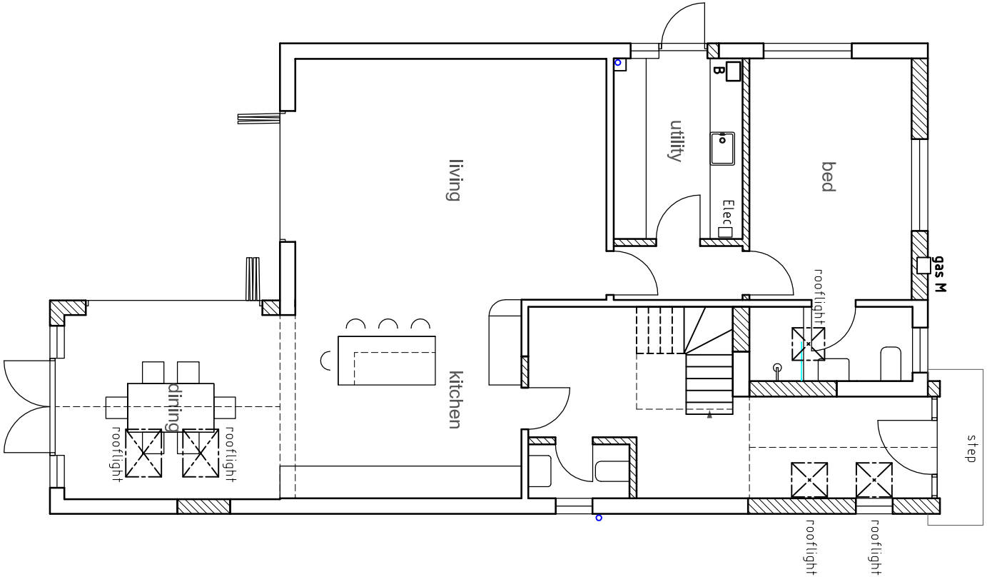
GROUND 1:100
