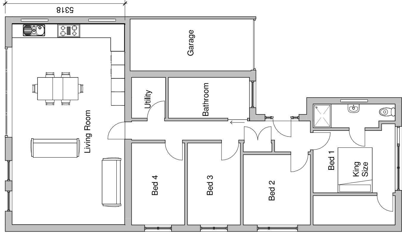
Proposed Ground Floor 1 : 100
